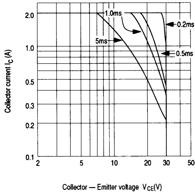
Figure 6 Reference Data Output Transistor ASO
