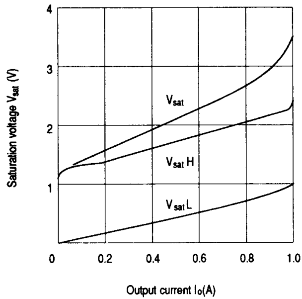
Figure 5 Reference Data Saturation Voltage vs. Output Current
