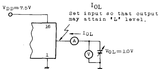
(9) Output current ("L" level)
